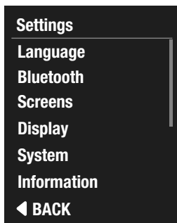
Fig. 8: Menu Settings
