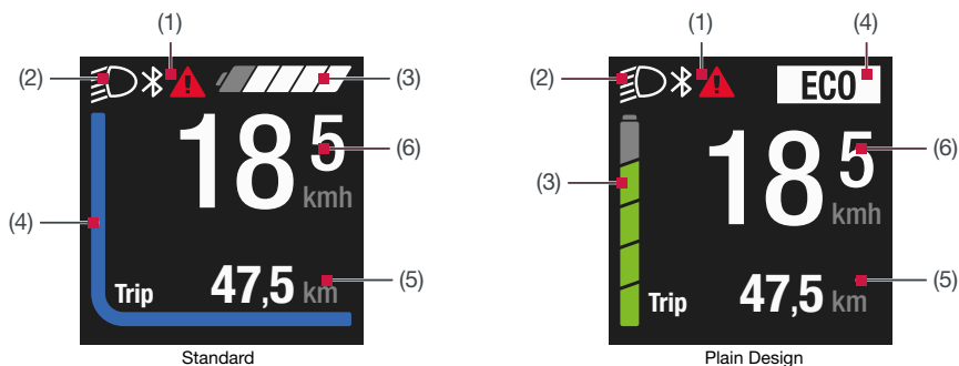
Fig. 2: User interface
